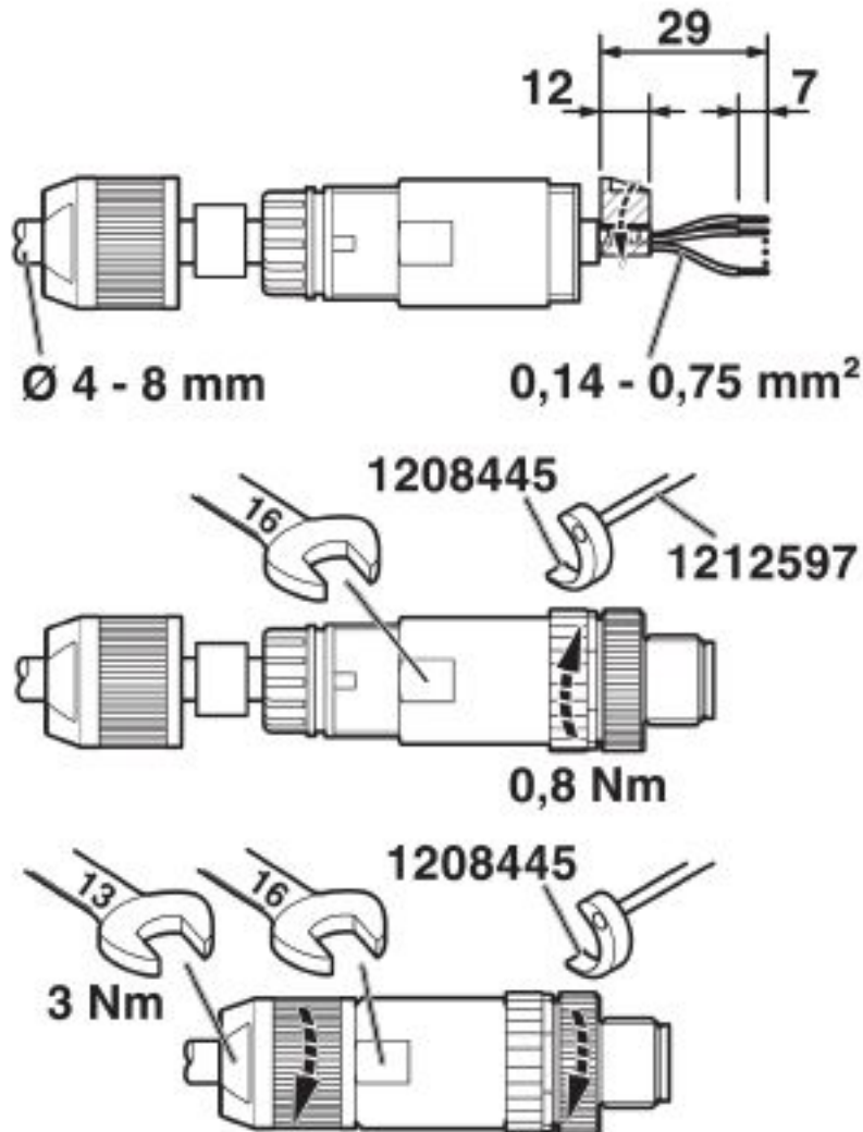
Functional drawing
