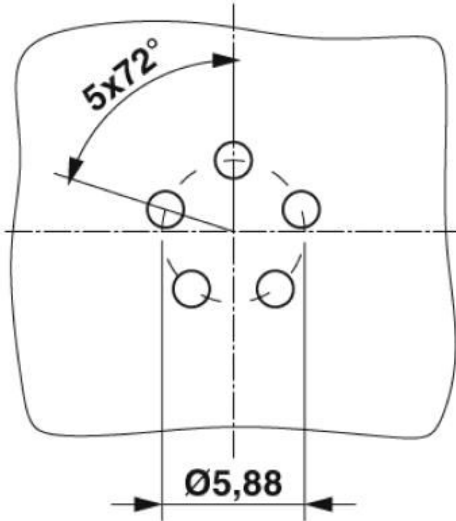
Drilling diagram
