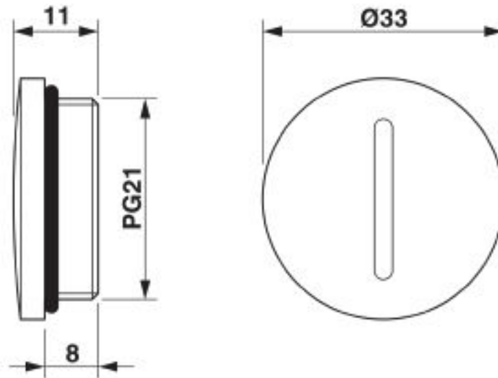
Dimensional drawing
