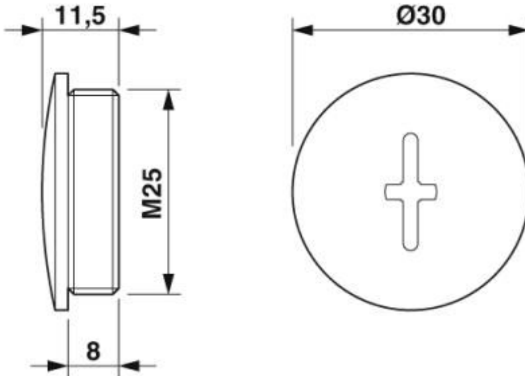
Dimensional drawing
