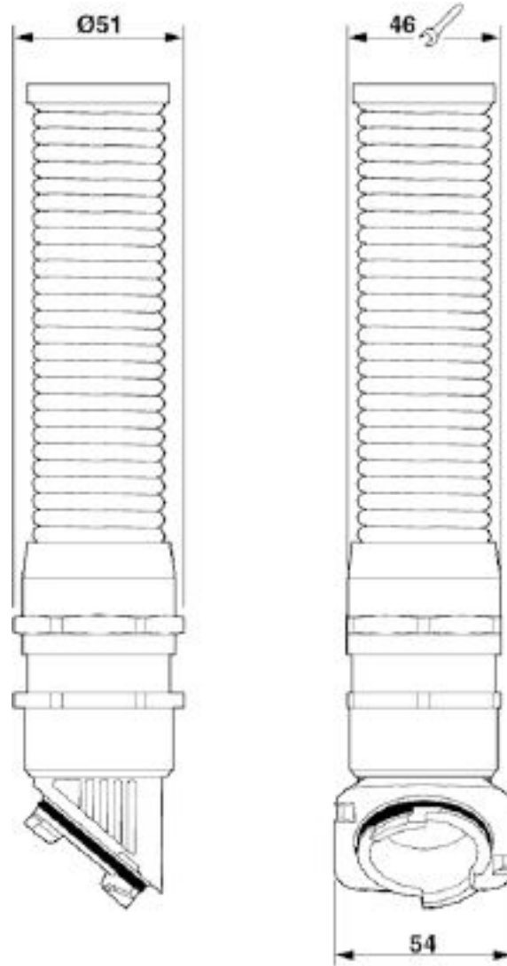
Dimensional drawing
