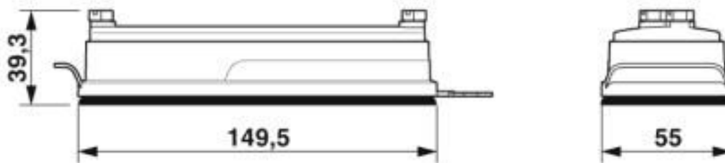
Dimensional drawing
