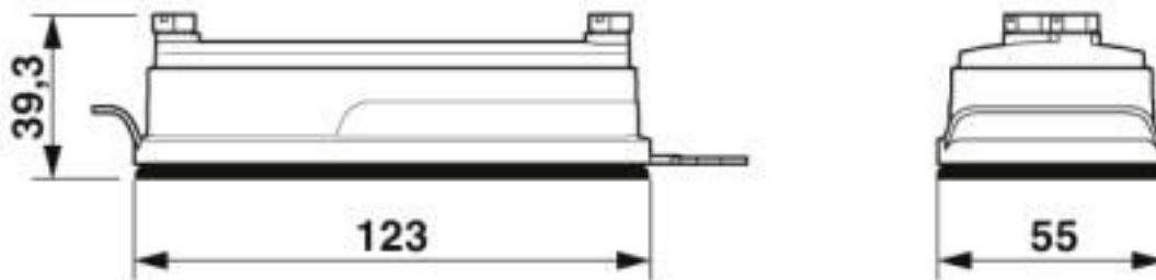
Dimensional drawing
