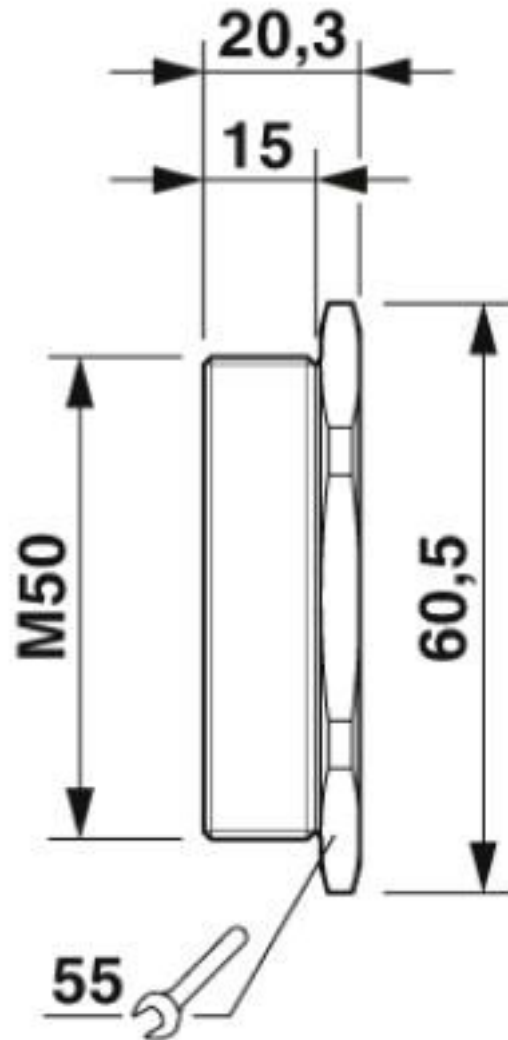
Dimensional drawing
