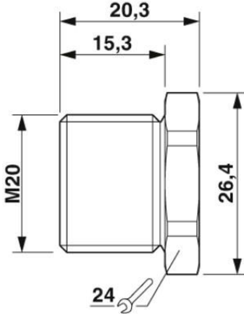
Dimensional drawing
