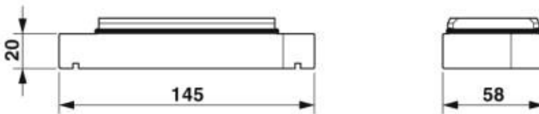
Dimensional drawing
