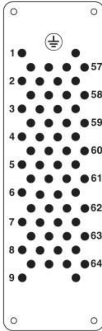
Schematic diagram
