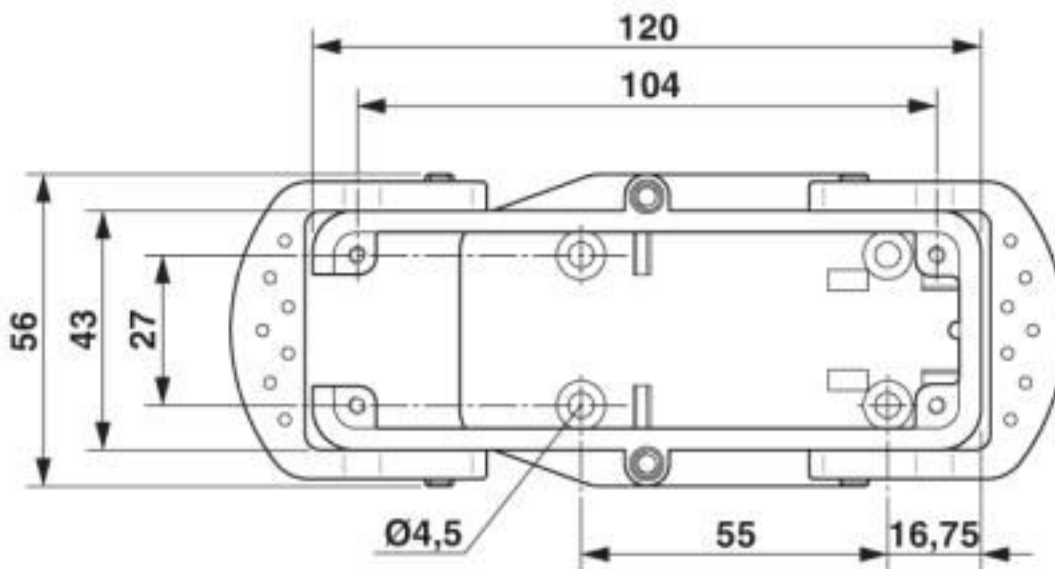
Dimensional drawing top view
