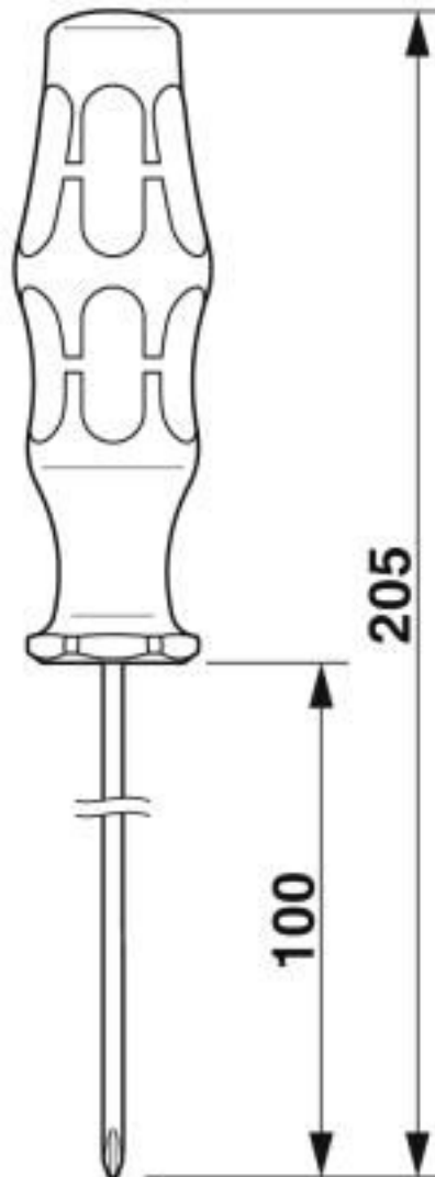
Dimensional drawing
